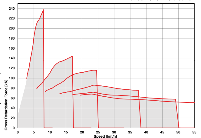
ADT, B35E 6X6 - Retardation
