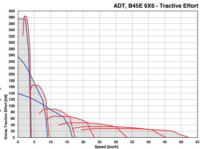
ADT, B45E 6X6 - Tractive Effort
