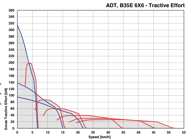
ADT, B35E 6X6 - Tractive Effort
